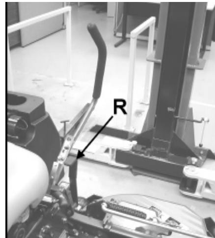
Parking brake in ON position (operator's left side)
